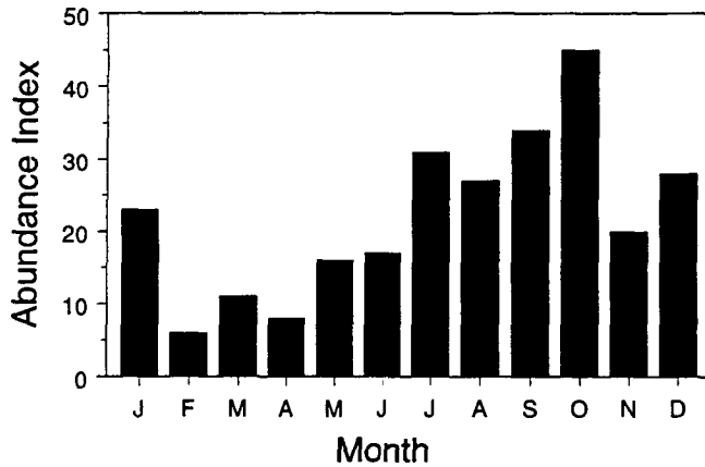
Figure 33 Monthly abundance (CPUE x 10) of all sizes of C. productus collected with the ringnets from 1983 to 1989
