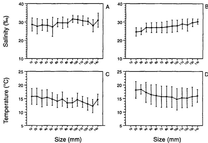
Figure 40 Mean salinity (%) and temperature (°C) ( \pm 1 standard deviation) for C. productus by size class collected with the otter trawl and ringnets: (A) salinity, otter trawl; (B) salinity, ringnets; (C) temperature, otter trawl; (D) temperature, ringnets. Size classes are every 10 mm, from 5 to 145 mm for the otter trawl, and 15 to 145 mm for the ringnets.
