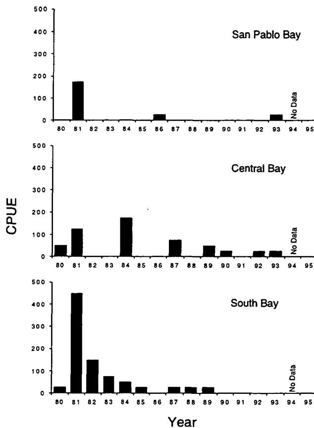
Figure 22 Annual distribution by bay of age-0 walleye surfperch collected with the midwater trawl from 1980 to 1995. Annual CPUE was May to August. Values are CPUE × 100.
