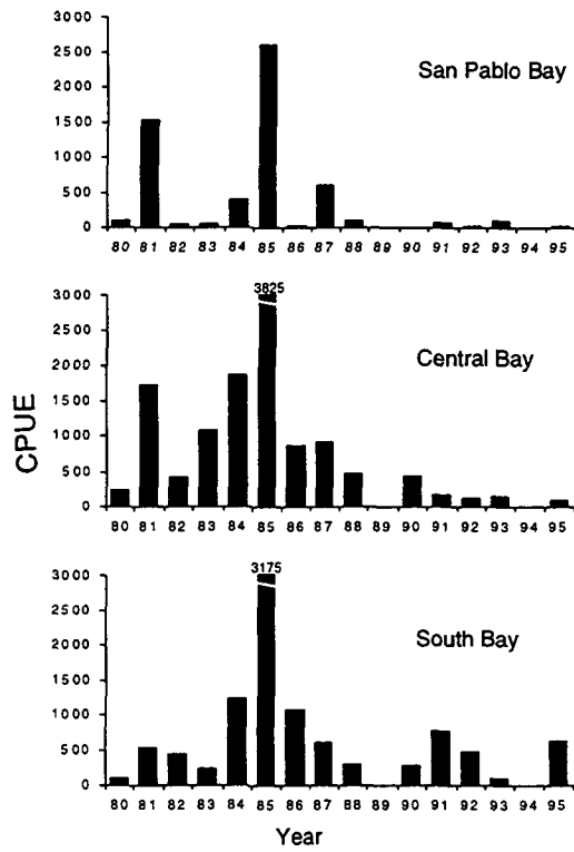
Figure 22 Annual distribution by region of age-0 jacksmelt collected with the midwater trawl from 1980 to 1995. Abundance index was July to October.
